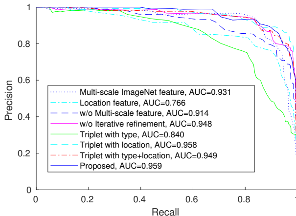
Figure 8. Precision-recall curves of various methods on the intra-patient lesion matching task using DeepLesion. The area-under-curve (AUC) values are shown in the legends.
